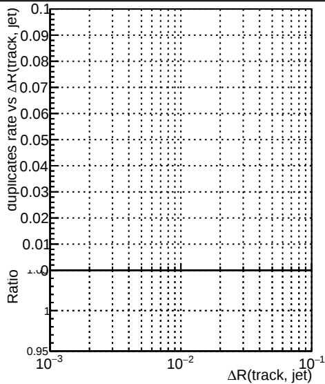
—●— DQM_V0001_R000000001_Global_mkFitbase_RECO —●— DQM_V0001_R000000001_Global_CMSSW_X_Y_Z_RECO
