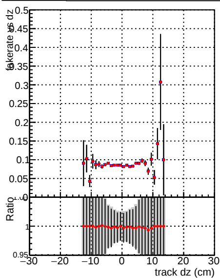
Fake rate vs d Legend: DQM_V0001_R0000000001_Global_mkFitbase_RECO DQM_V0001_R0000000001_Global_CMSSW_X_Y_Z_RECO
