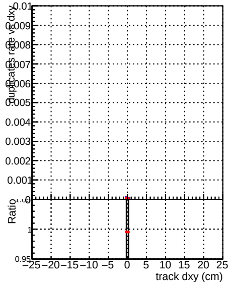
Global mkFitbase RECO Fake rate vs d DQM V0001_R0000000001 DQM V0001_R0000000001 DQM V0001_R0000000001 Duplicates rate vs d DQM V0001_R0000000001 DQM V0001_R0000000001 DQM V0001_R0000000001 Pileup rate vs d DQM V0001_R0000000001 DQM V0001_R0000000001 DQM V0001_R0000000001
