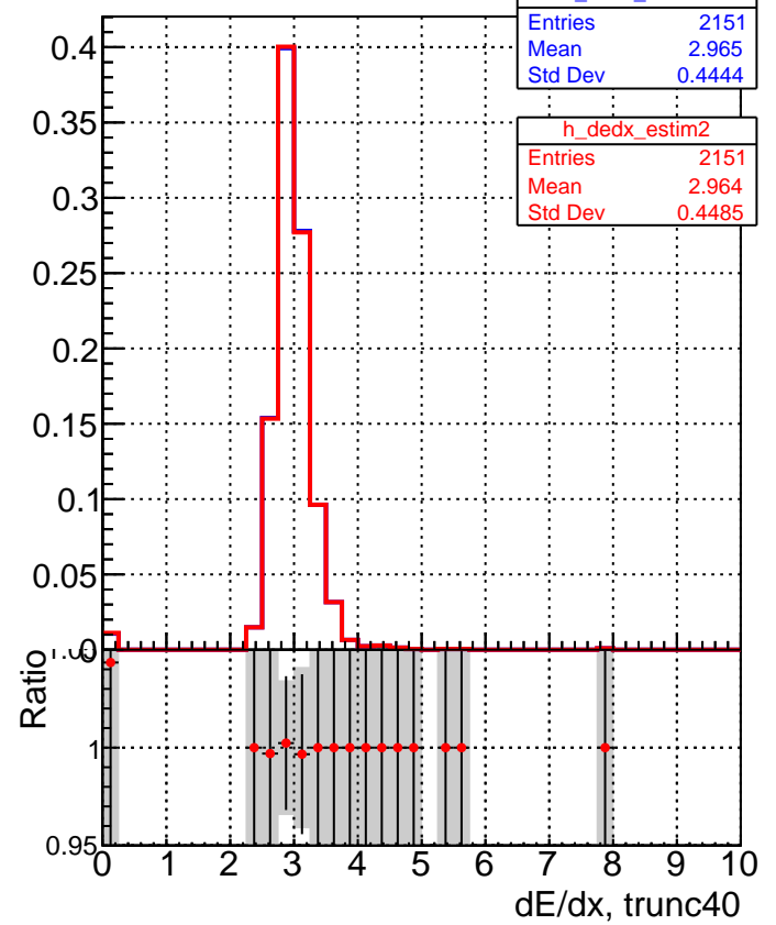
■ DQM_V0001_R000000001_Global_mkFitbase_RECO ● DQM_V0001_R000000001_Global_CMSSW_X_Y_Z_RECO
