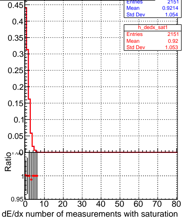
■ DQM_V0001_R000000001_Global_mkFitbase_RECO ● DQM_V0001_R000000001_Global_CMSSW_X_Y_Z_RECO
