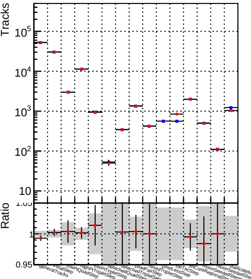
DQM_V0001_R000000001_Global_mkFitbase_RECO
