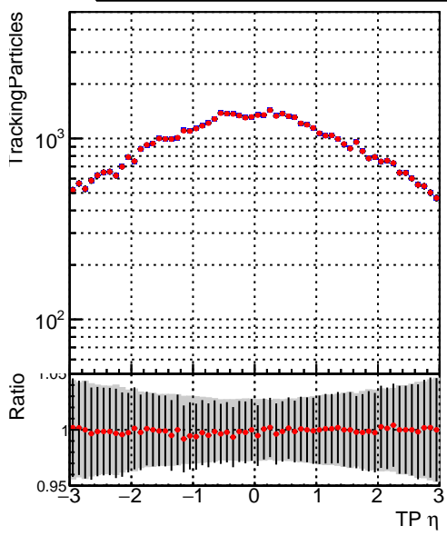
N of simulated tracks vs \eta Legend: \blacksquare DQM_V0001_R000000001_Global_mkFitbase_RECO \bullet DQM_V0001_R000000001_Global_CMSSW_X_Y_Z_RECO
