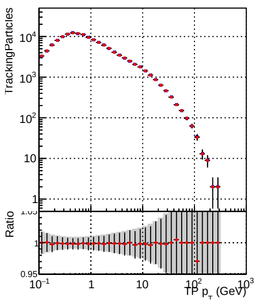
Legend: DQM_V0001_R000000001_Global_mkFitbase_RECO (blue line with markers), DQM_V0001_R000000001_Global_CMSSW_X_Y_Z_RECO (red line with markers)
