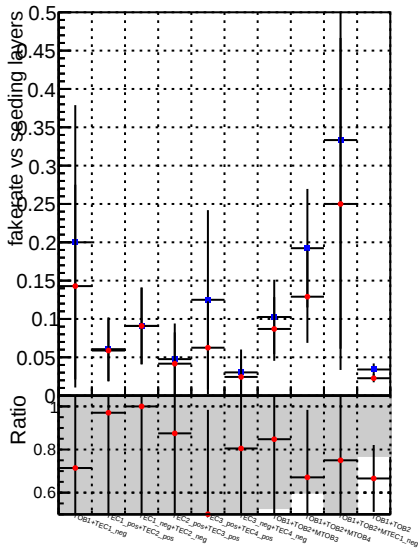
Fake rate vs. —•— DQM_V0001_R0000000001_Global_mkFitbase_RECO —•— DQM_V0001_R0000000001_Global_CMSSW_X_Y_Z_RECO
