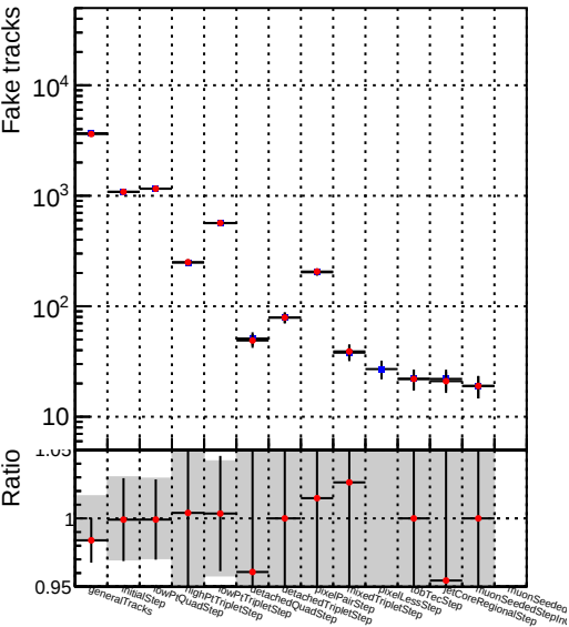
Number —●— DQM_V0001_R000000001_Global_CMSSW_X_Y_Z_RECO
