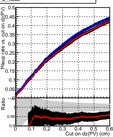
DQM_V0001_R000000001_Global_CMSSW_X_Y_Z_RECO
