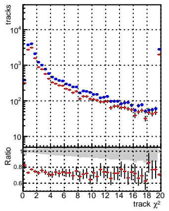
N of reco track vs. - blue circles: DQM_V0001_R000000001_Global_mkFitbase_RECO - red circles: DQM_V0001_R000000001_Global_CMSSW_X_Y_Z_RECO
