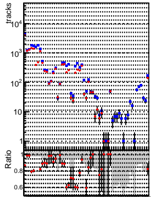
N of reco track vs. - blue circles: DQM_V0001_R000000001_Global_mkFitbase_RECO - red circles: DQM_V0001_R000000001_Global_CMSSW_X_Y_Z_RECO
