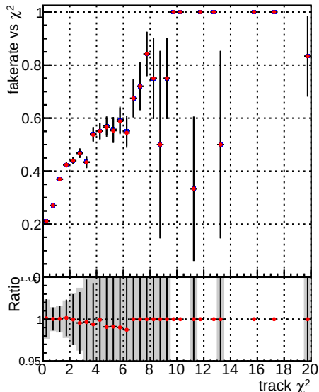
Fake rate vs. \chi^2 Legend: Global mkFitbase RECO (Blue line with error bars) Global CMSSW X Y Z RECO (Red line with error bars)
