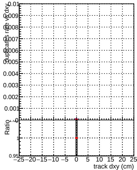
Global mkFitbase RECO Fake rate vs d DQM_V0001_R000000001 DQM_V0001_R000000001 DQM_V0001_R000000001 Duplicates rate vs d DQM_V0001_R000000001 DQM_V0001_R000000001 DQM_V0001_R000000001 Pileup rate vs d DQM_V0001_R000000001 DQM_V0001_R000000001 DQM_V0001_R000000001
