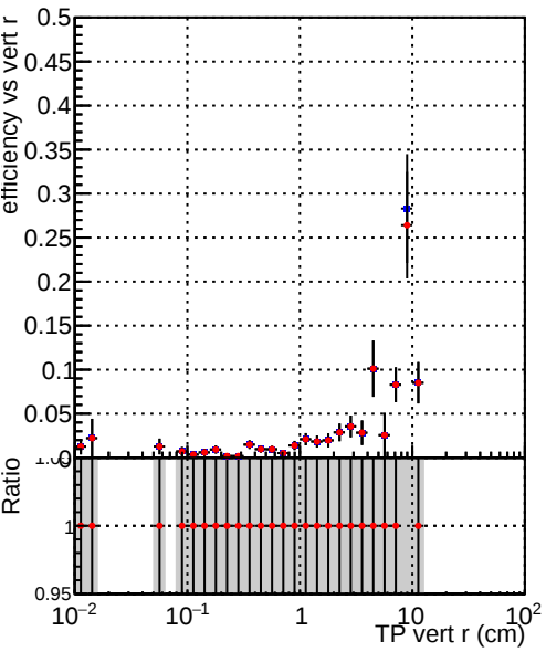
Efficiency vs vertpos Legend: DQM_V0001_R000000001_Global_mkFitbase_RECO DQM_V0001_R000000001_Global_CMSSW_X_Y_Z_RECO
