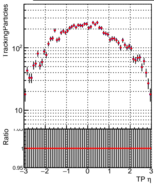
N of simulated tracks vs TP \eta Legend: — DQM_V0001_R000000001_Global_mkFitbase_RECO (blue line) — DQM_V0001_R000000001_Global_CMSSW_X_Y_Z_RECO (red line)
