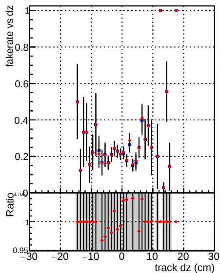
DQM_V0001_R0000000001_Global_mkFitbase_RECO Fake rate vs d DQM_V0001_R0000000001_Global_CMSSW_X_Y_Z_RECO
