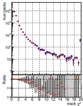
N of reco track vs. \chi^2 for DQM V0001_R000000001 and Global_mkFitbase_RECO.
