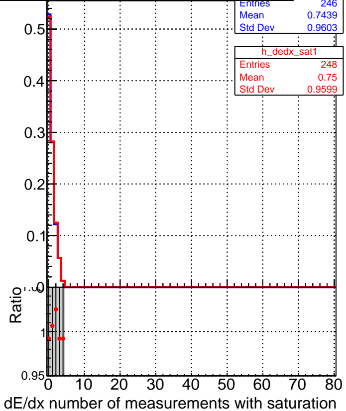
■ DQM_V0001_R000000001_Global_mkFitbase_RECO ● DQM_V0001_R000000001_Global_CMSSW_X_Y_Z_RECO
