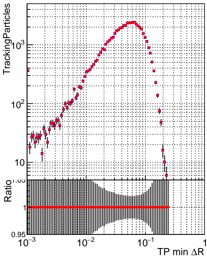
■ DQM_V0001_R000000001_Global_mkFitbase_RECO ● DQM_V0001_R000000001_Global_CMSSW_X_Y_Z_RECO
