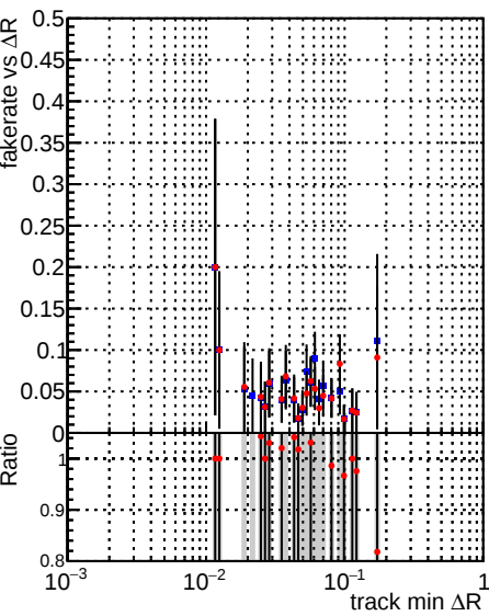
Fake rate vs \Delta R(\text{track}, \text{jet}) DQM_V0001_R000000001_Global_mkFitbase_RECO DQM_V0001_R000000001_Global_CMSSW_X_Y_Z_RECO
