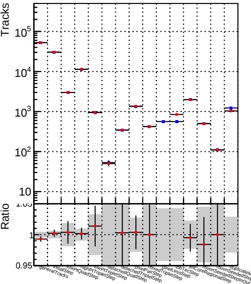
DQM_V0001_R0000000001_Global_mkFitbase_RECO
