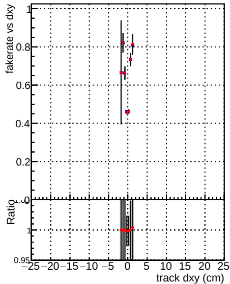
Global mkFitbase RECO —●— DQM V0001_R0000000001 —●— DQM V0001_R0000000001
