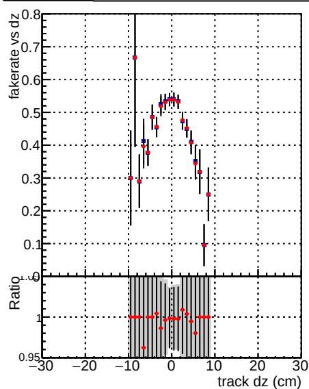
Global mkFitbase RECO —●— DQM V0001_R0000000001 —●— DQM V0001_R0000000001
