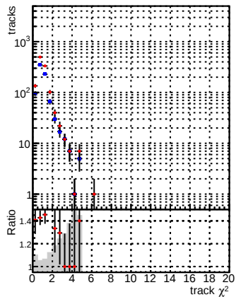
N of reco track vs. \chi^2 for DQM V0001 R000000001 Global mkFitbase RECO and DQM V0001 R000000001 Global CMSSW X_Y_Z_RECO
