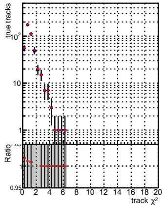
Legend: Global mkFitbase RECO Global CMSSW X_Y_Z RECO
