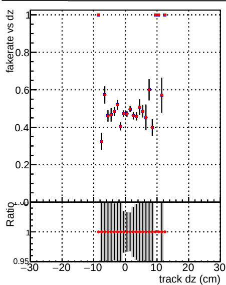
Fake rate vs dz DQM_V0001_R0000000001 Global mkFitbase RECO DQM_V0001_R0000000001 Global mkSSW_X_Y_Z RECO
