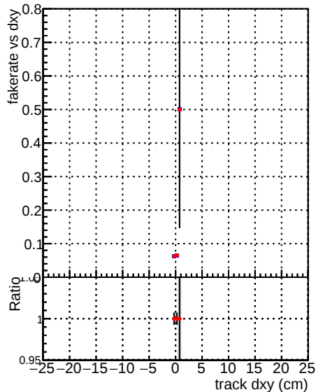
—●— DQM_V0001_R000000001 Global mkFitbase RECO —●— DQM_V0001_R000000001 Global CMSSW X Y Z RECO
