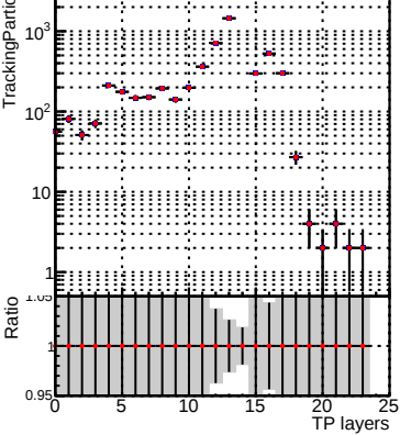
N of simulated tracks vs pixel layer
