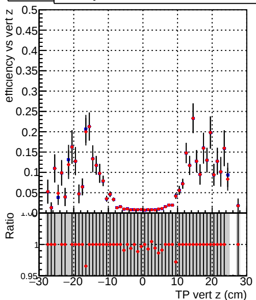
Efficiency vs TP vert z — DQM_V0001_R000000001_Global_mkFitbase_RECO — DQM_V0001_R000000001_Global_CMSSW_X_Y_Z_RECO
