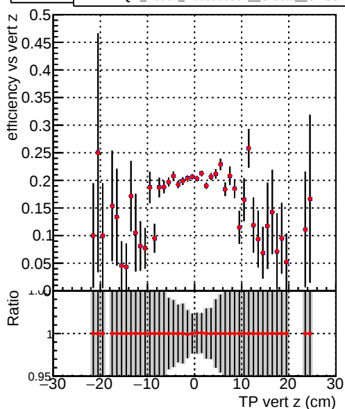
Efficiency vs vert z — DQM_V0001_R000000001_Global_mkFitbase_RECO — DQM_V0001_R000000001_Global_CMSSW_X_Y_Z_RECO
