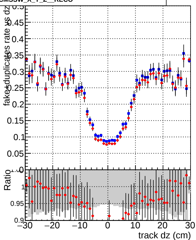
—■— DQM_V0001_R000000001_Global_mkFitbase_RECO —●— DQM_V0001_R000000001_Global_CMSSW_X_Y_Z_RECO
