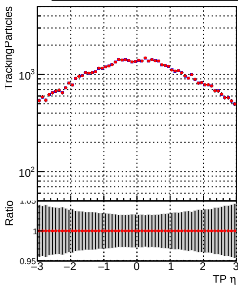
Legend: DQM_V0001_R000000001_Global_mkFitbase_RECO (blue squares), DQM_V0001_R000000001_Global_CMSSW_X_Y_Z_RECO (red diamonds)
