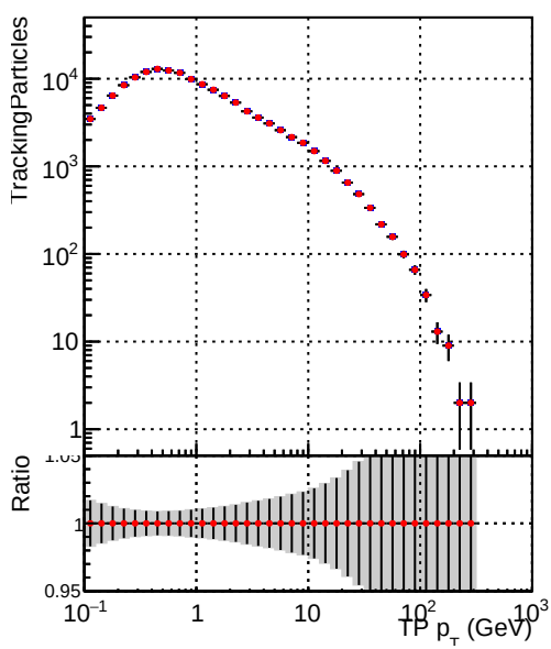
Legend: DQM_V0001_R000000001_Global_mkFitbase_RECO (blue squares), DQM_V0001_R000000001_Global_CMSSW_X_Y_Z_RECO (red diamonds)
