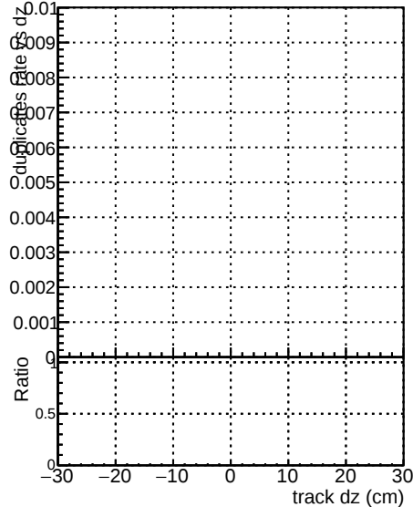
—●— DQM_V0001_R0000000001_Global_mkFitbase_RECO —●— DQM_V0001_R0000000001_Global_CMSSW_X_Y_Z_RECO
