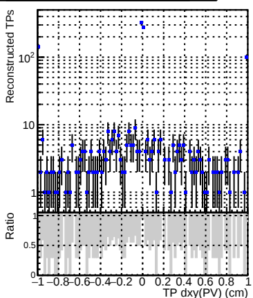
DQM_V0001_R000000001_Global_mkFitbase_RECO
