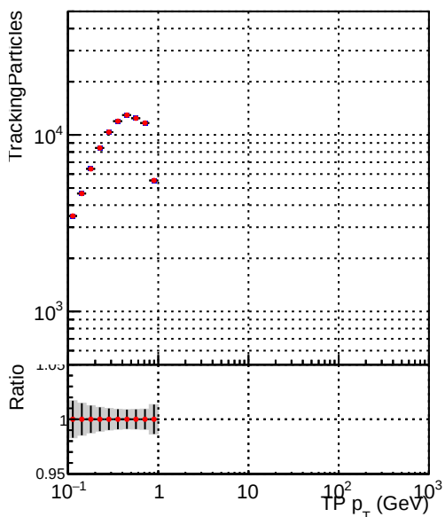
—•— DQM_V0001_R0000000001_Global_mkFitbase_RECO —•— DQM_V0001_R0000000001_Global_CMSSW_X_Y_Z_RECO
