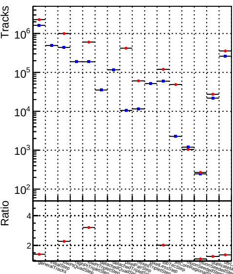
DQM_V0001_R000000001_Global_mkFitbase_RECO
