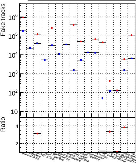
Number DQM_V0001_R000000001_Global_CMSSW_X_Y_Z_RECO
