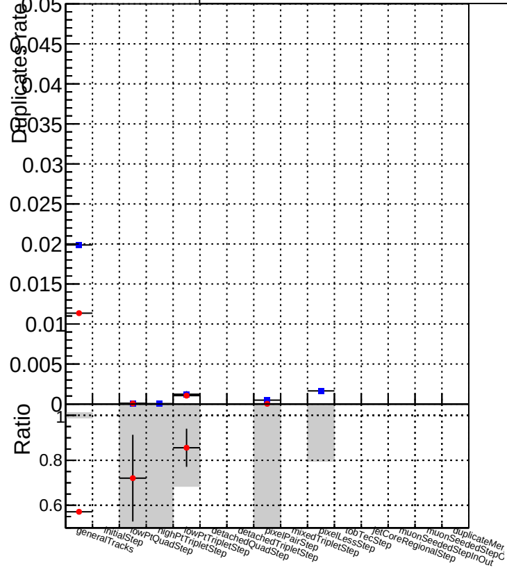
Duplicates rate vs collection Legend: Global_mkFitbase_RECO (blue squares) Global_CMSSW_X_Y_Z_RECO (red circles)
