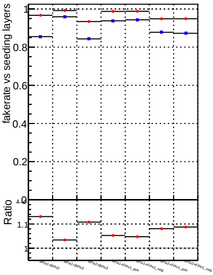
Fake rate vs. DQM_V0001_R000000001_Global_mkFitbase_RECO DQM_V0001_R000000001_Global_mkSSW_X_Y_Z_RECO
