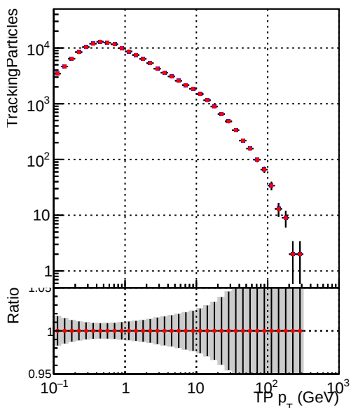
—•— DQM_V0001_R0000000001_Global_mkFitbase_RECO —•— DQM_V0001_R0000000001_Global_CMSSW_X_Y_Z_RECO
