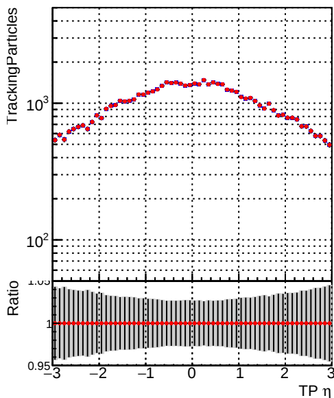
—•— DQM_V0001_R0000000001_Global_mkFitbase_RECO —•— DQM_V0001_R0000000001_Global_CMSSW_X_Y_Z_RECO
