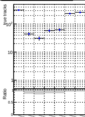
Legend: - Blue dots: DQM_V0001_R000000001_Global_mkFitbase_RECO - Grey shaded: DQM_V0001_R000000001_Global_CMSSW_X_Y_Z_RECO
