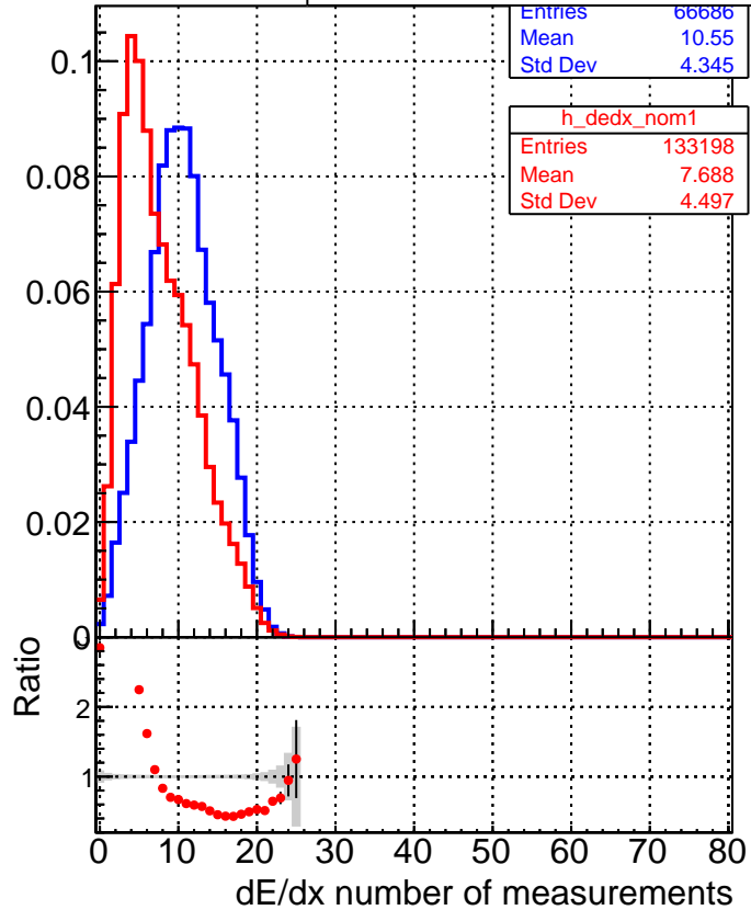
—■ DQM_V0001_R000000001_Global_mkFitbase_RECO —● DQM_V0001_R000000001_Global_CMSSW_X_Y_Z_RECO
