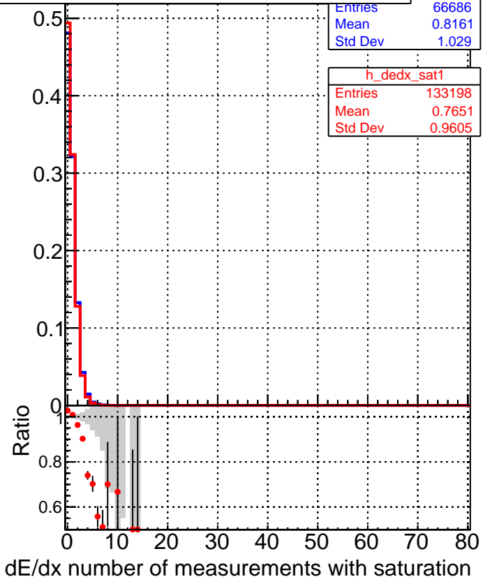
—■ DQM_V0001_R000000001_Global_mkFitbase_RECO —● DQM_V0001_R000000001_Global_CMSSW_X_Y_Z_RECO
