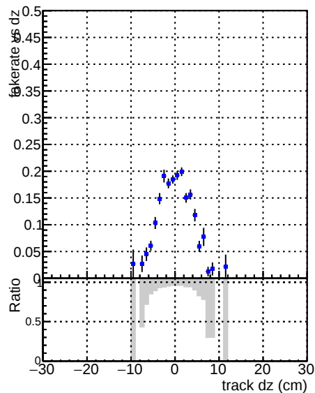
Fake rate vs dz Legend: Blue squares: DQM V0001_R000000001 Global mkFitbase RECO Red circles: DQM V0001_R000000001 Global mkSSW X Y Z RECO
