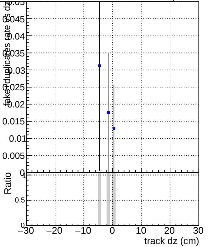
DQM_V0001_R000000001_Global_mkFitbase_RECO DQM_V0001_R000000001_Global_CMSSW_X_Y_Z_RECO
