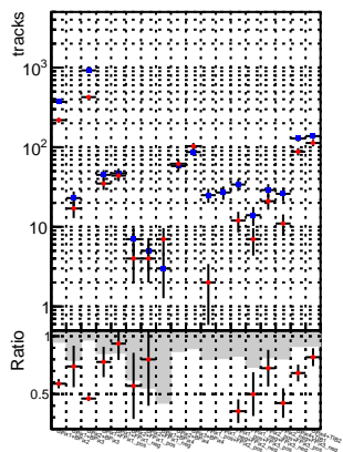
N of reco track vs. \chi^2 Global mkFitbase RECO Global CMSSW X_Y_Z RECO
