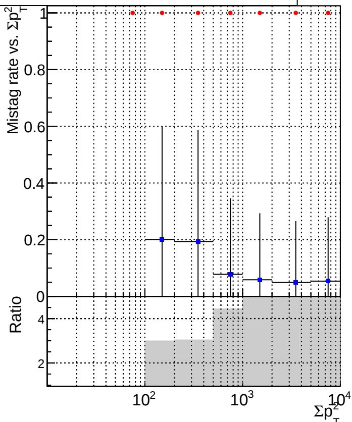
DQM_V0001_R000000001_Global_mkFitbase_RECO DQM_V0001_R000000001_Global_CMSSW_X_Y_Z_RECO
