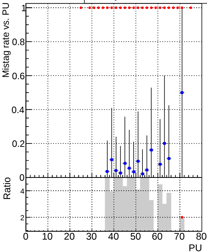
DQM_V0001_R000000001_Global_mkFitbase_RECO DQM_V0001_R000000001_Global_CMSSW_X_Y_Z_RECO
