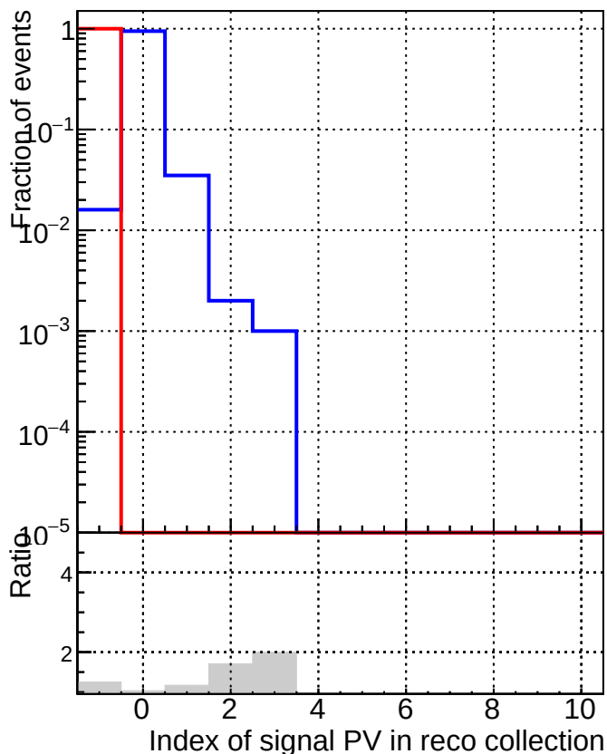
DQM_V0001_R000000001_Global_mkFitbase_RECO DQM_V0001_R000000001_Global_CMSSW_X Y Z_RECO
