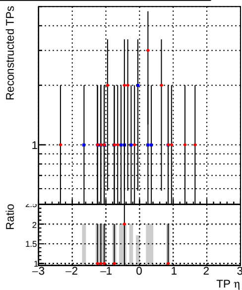
Legend: DQM_V0001_R000000001_Global_mkFitbase_RECO (blue line), DQM_V0001_R000000001_Global_CMSSW_X_Y_Z_RECO (red line)
