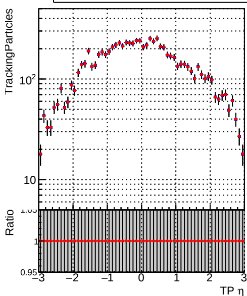
N of simulated tracks vs \eta Legend: DQM_V0001_R000000001_Global_mkFitbase_RECO (blue squares), DQM_V0001_R000000001_Global_CMSSW_X_Y_Z_RECO (red circles)
