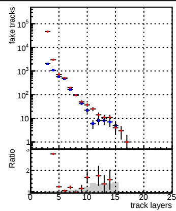
Legend: DQM_V0001_R000000001_Global_mkFitbase_RECO (blue circles), DQM_V0001_R000000001_Global_CMSSW_X_Y_Z_RECO (red line)
