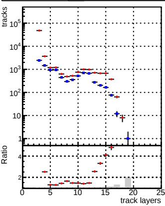
Legend: DQM_V0001_R000000001_Global_mkFitbase_RECO (blue circles), DQM_V0001_R000000001_Global_CMSSW_X_Y_Z_RECO (red line)
