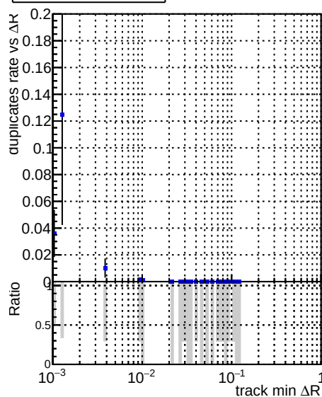
—•— DQM_V0001_R000000001_Global_mkFitbase_RECO —•— DQM_V0001_R000000001_Global_CMSSW_X_Y_Z_RECO
