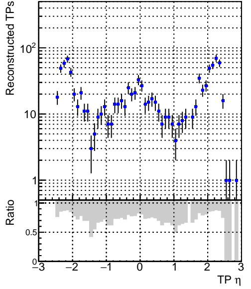
■ DQM_V0001_R000000001_Global_mkFitbase_RECO ■ DQM_V0001_R000000001_Global_CMSSW_X_Y_Z_RECO
